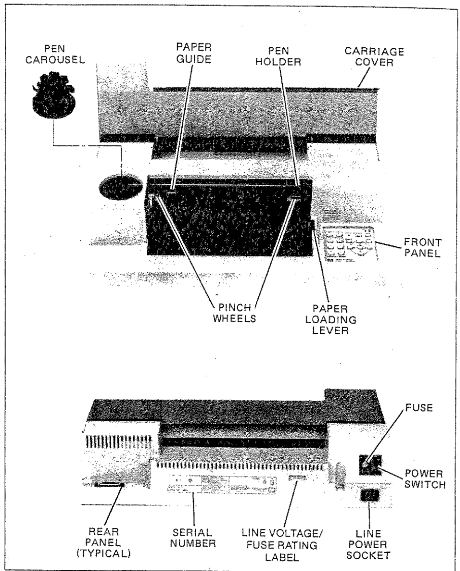
Major Feature Locations
