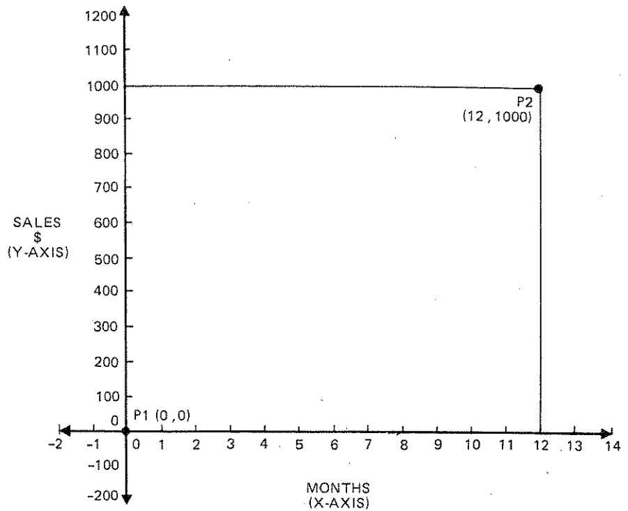
User-Unit Scaling
