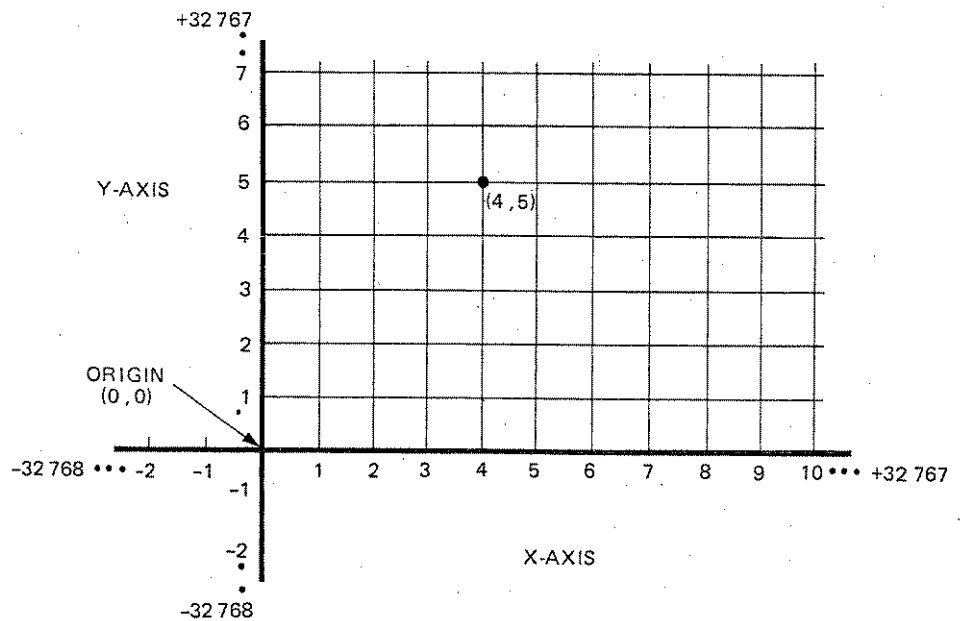
Cartesian Coordinates
